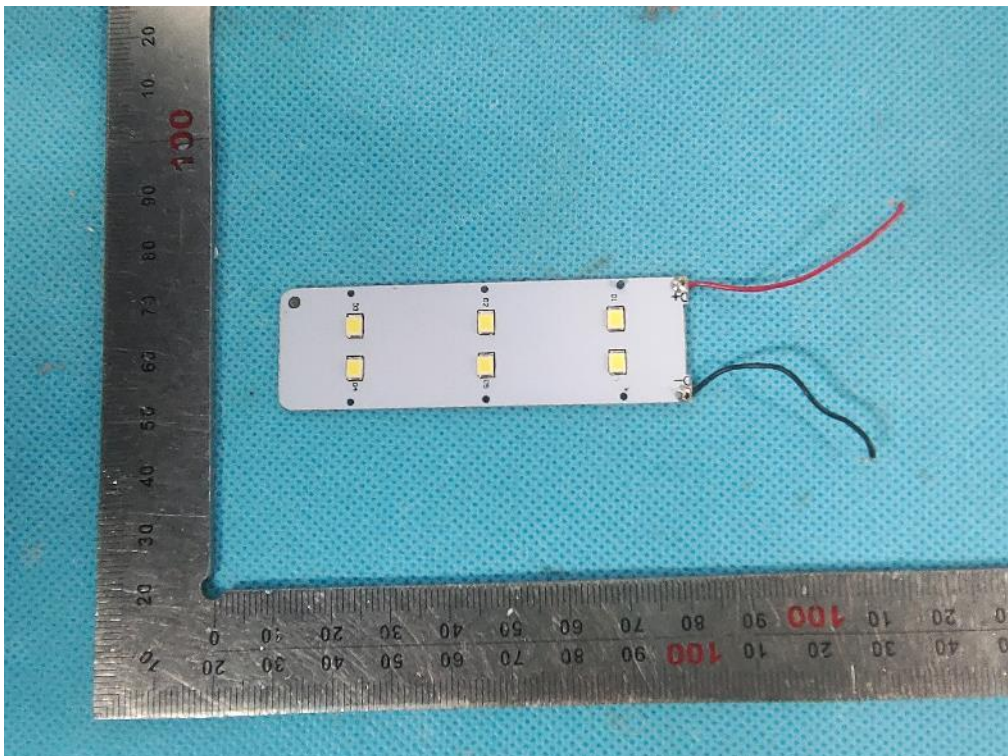
Fig. 10 – LED view
